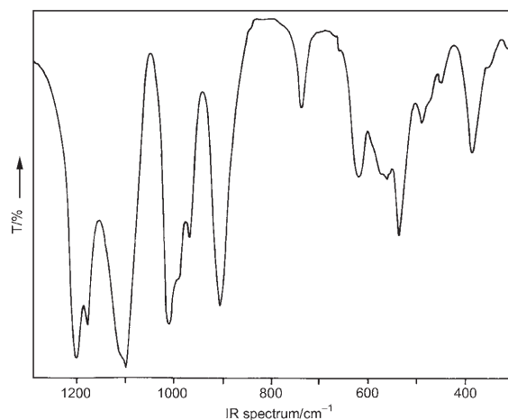
Fig. 1 Infrared spectrum of \text{Na}_6[(\text{VO})_3(\text{P}_2\text{O}_7)_3]\cdot 7\text{H}_2\text{O} , between 1300 and 300 \text{cm}^{-1}
